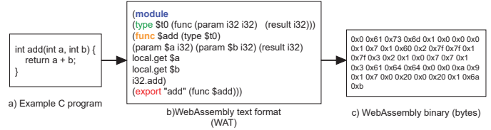
Fig. 1. Wasm example; a simple C function (left) compiled into the Wasm (middle and right). local.get and i32.add are the opcode of the instructions, and $a and $b are the immediate arguments.
